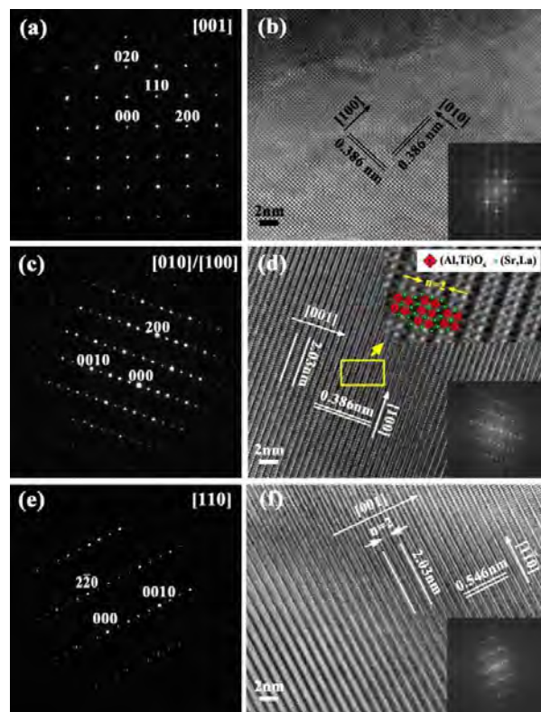
Fig. 6 SAED patterns and corresponding HRTEM images in [001], [010], [110] zone axis for \text{Sr}_2\text{LaAlTiO}_7 ceramics. The simulated diffraction pattern of HRTEM images using FFT are also shown in the inset.
